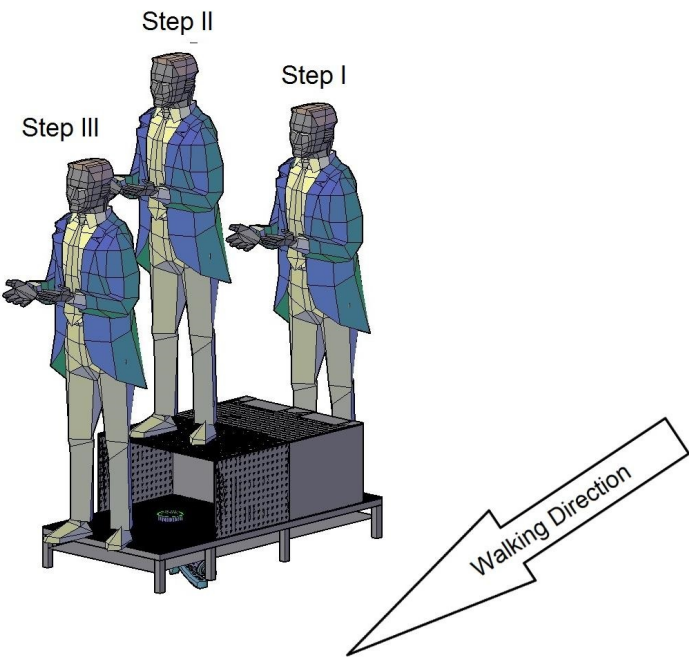
Three steps walk through footwear sanitization system
